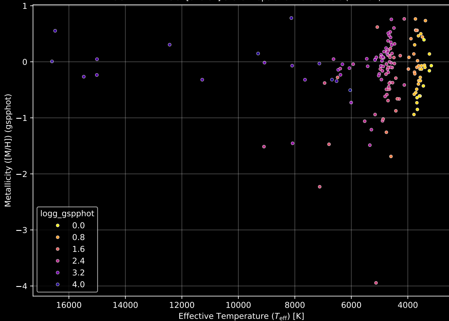
APOGEE DR17 Field: [010-02] Stellar Population Parameters (n= 152)
