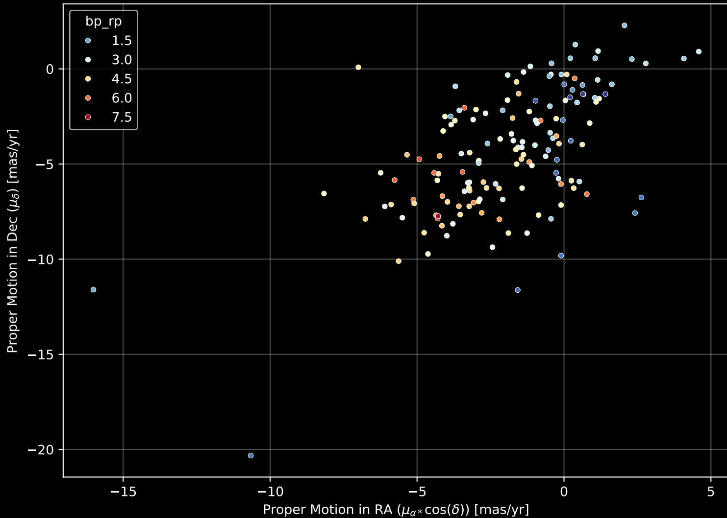
APOGEE DR17 Field: [010-02] Proper Motion Diagram (n= 152)
