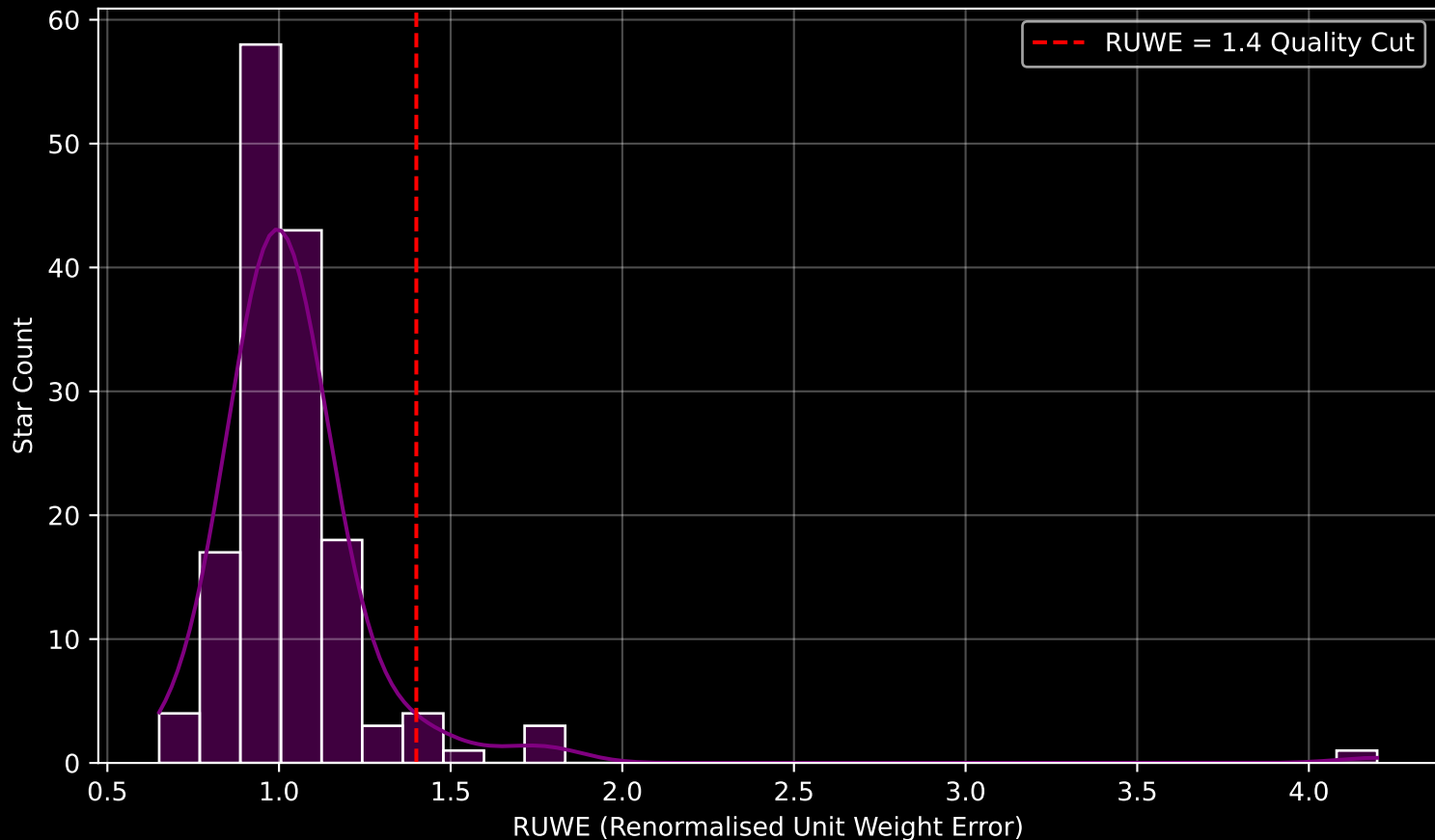
GAPOGEE DR17 Field [010-02] RUWE Distribution (n= 152)
