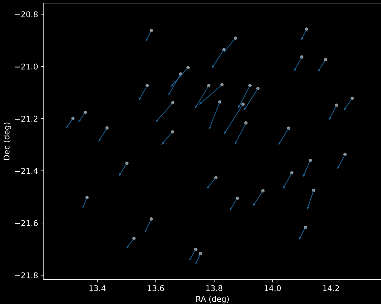
APOGEE DR17 Cluster 0 Proper Motion Vectors (n=38)
