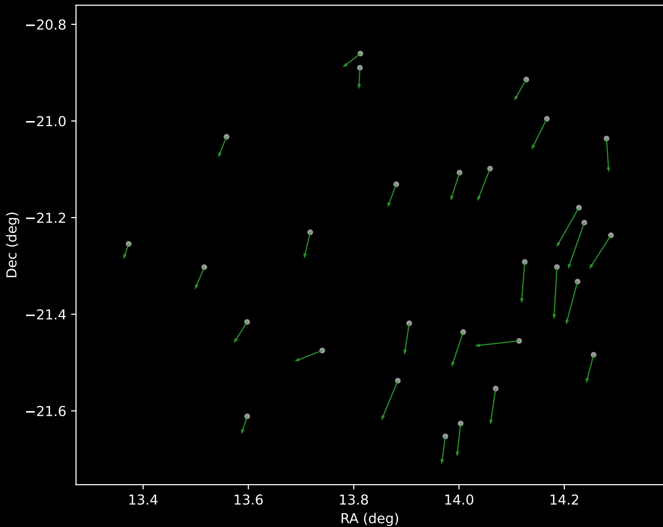
APOGEE DR17 Cluster 4 Proper Motion Vectors (n=29)
