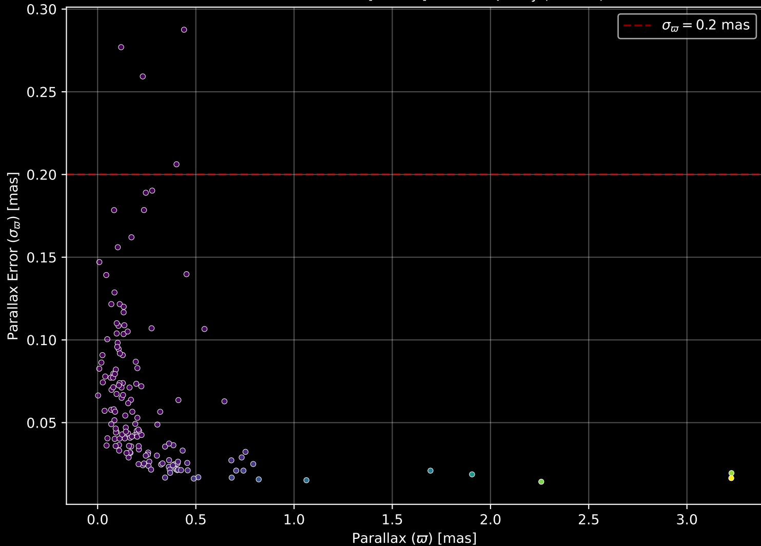
APOGEE DR17 Field: [010-02] Parallax Quality (n= 152)
