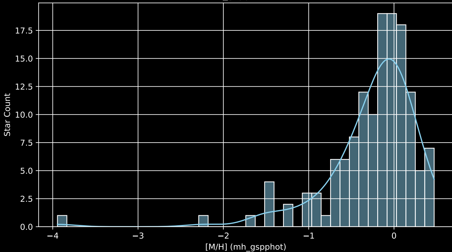
APOGEE DR17 Field: [010-02 [M/H] (mh_gspphot) (n= 138)
